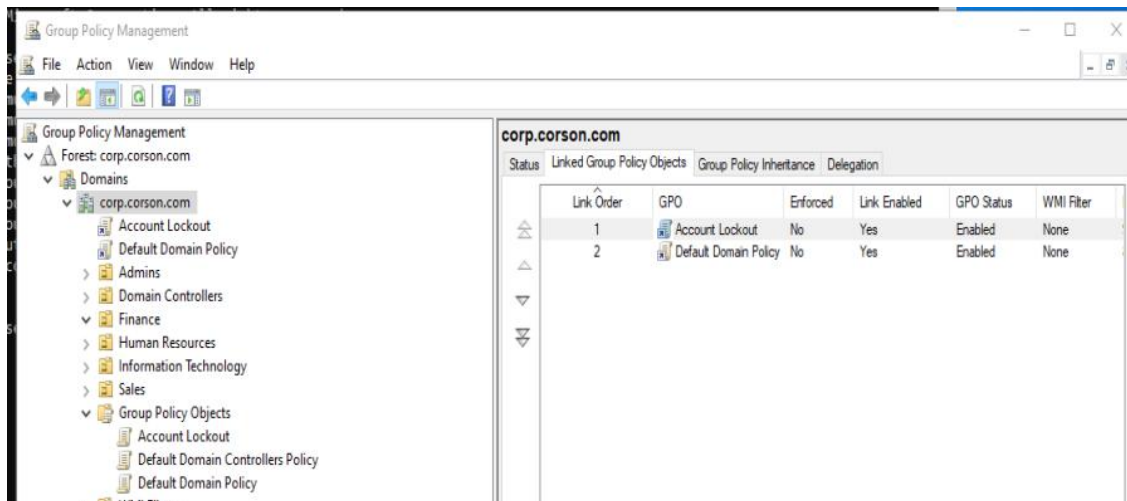
Figure 7. Established Linked Account Lockout GPO precedence is being set as the number 1 priority, allowing the new GPO to take precedence over the default linked Domain policy.
