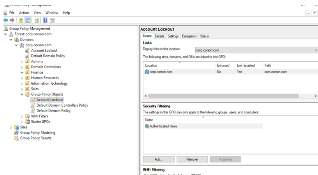
Figure 6. Figure Displays successful verification of corp.corson.com enterprise being linked to the Account Lockout GPO.
