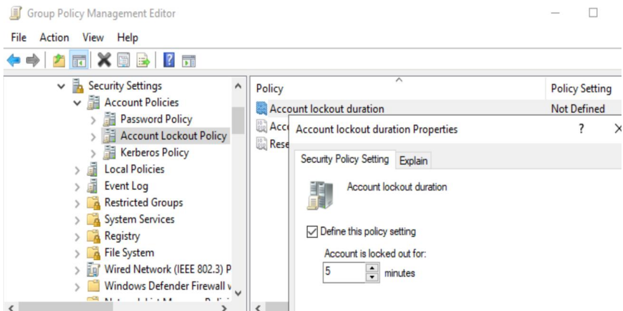
Figure 3. “Account Lockout” GPO is being configured with policies that will define the conditions it will operate under. Example shows that 5 minutes will be placed on account that violates conditions.
