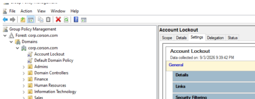
Figure 5. Created “Account Lockout” GPO is linked under the corp.corson.com enterprise, process is configuring lockout policy to globally effect users under the enterprise.
