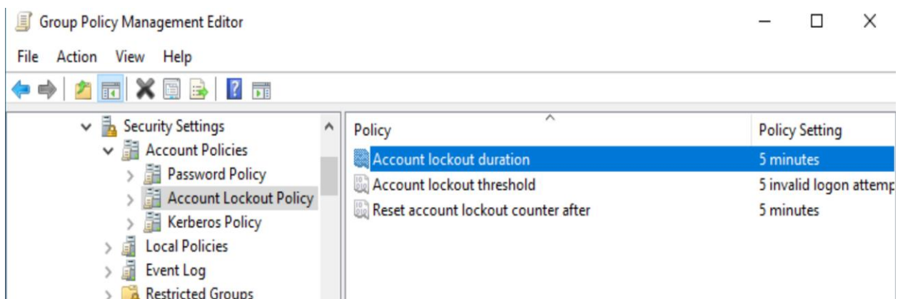
Figure 4. Figure continues defining Account Lockout GPO, example shows that after five invalid user login attempts, account will be locked for 5 minutes.
